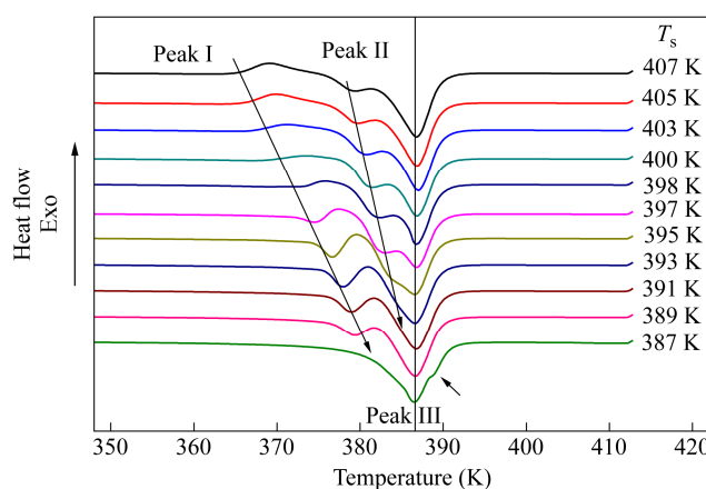
Fig. 3 Subsequent DSC heating curves (at 10 K/min) after controlled cooling scans shown in Fig. 2(a)
